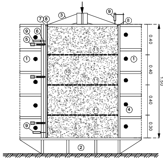
Figure 6. Test setup with movable front wall (Bussert 2006)
