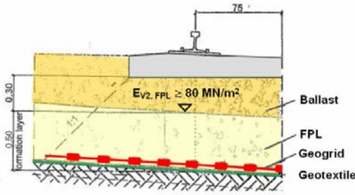
Figure 9. Standard Cross Section of FPL (Formation Protection Layer)
