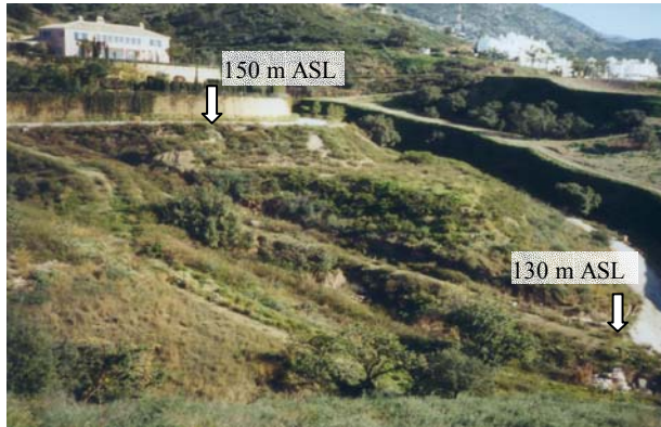
Figure 20. Original site situations in the hills of Marbella / Spain
