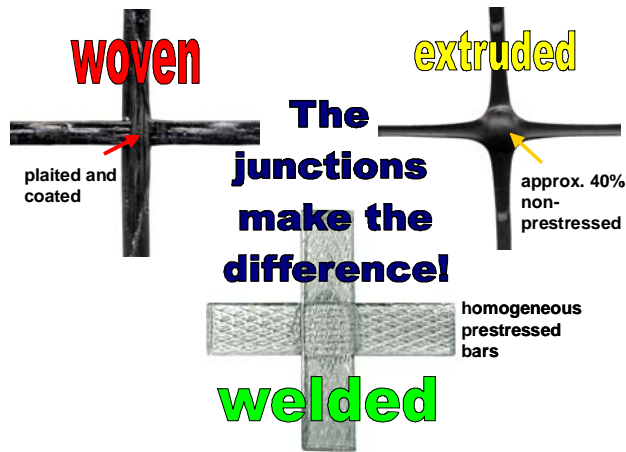
Figure 5. Different junction design of existing geogrid products
