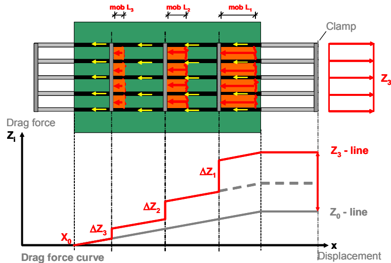
Figure 4. Mobilization of friction and soil resistance by pull-out of a geogrid
